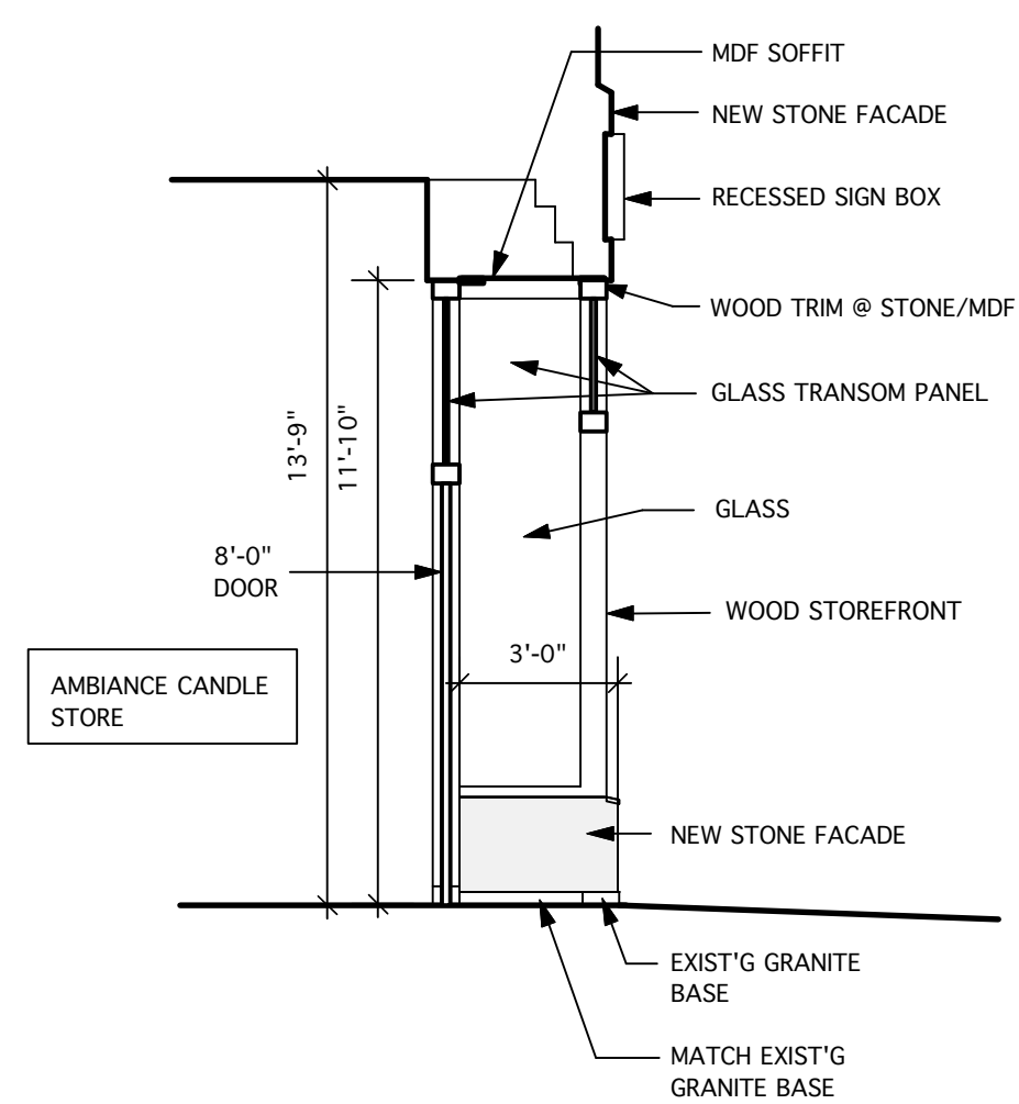
ELEVATION- SIDE WALL SCALE: 1/4"= 1'-0"
