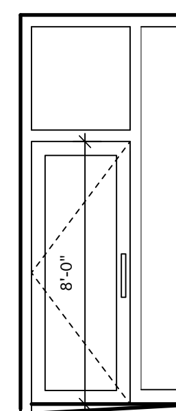
ELEVATION- DOOR OF SIDE DOOR SCALE: 1/4"= 1'-0"
